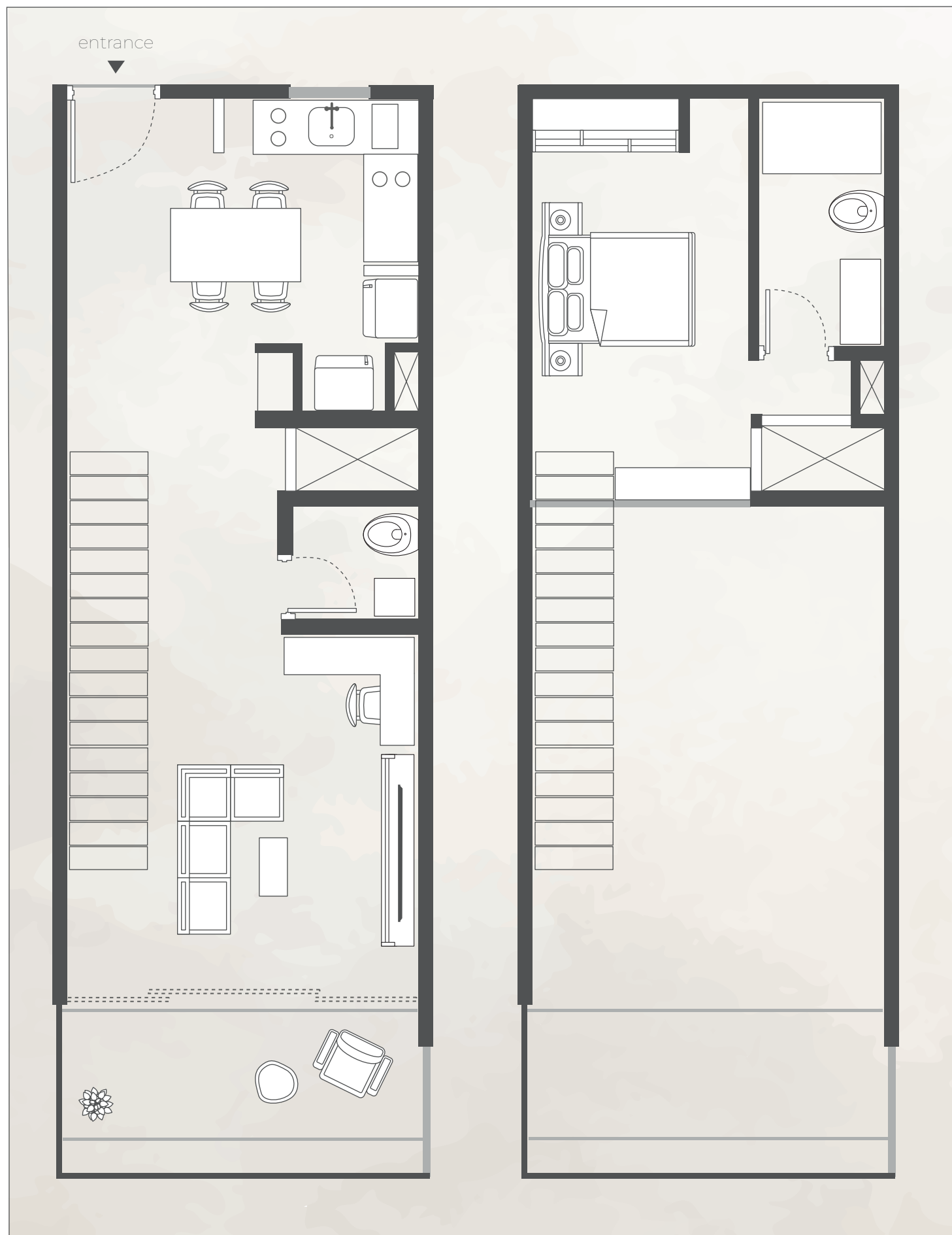
FIRST FLOOR scale 1: 25
